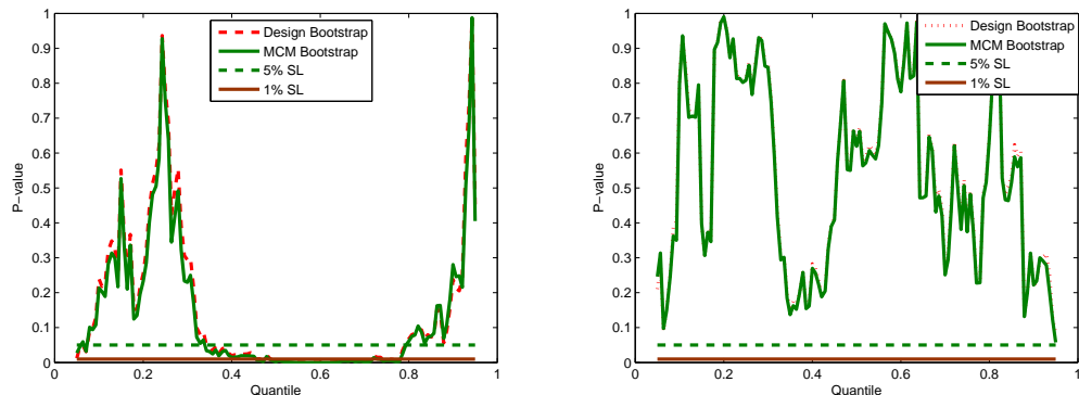
(a) P-values of the impact of anticipated unem- (b) P-values of the impact of unanticipated un- ployment rate on stock return employment rate on stock return
